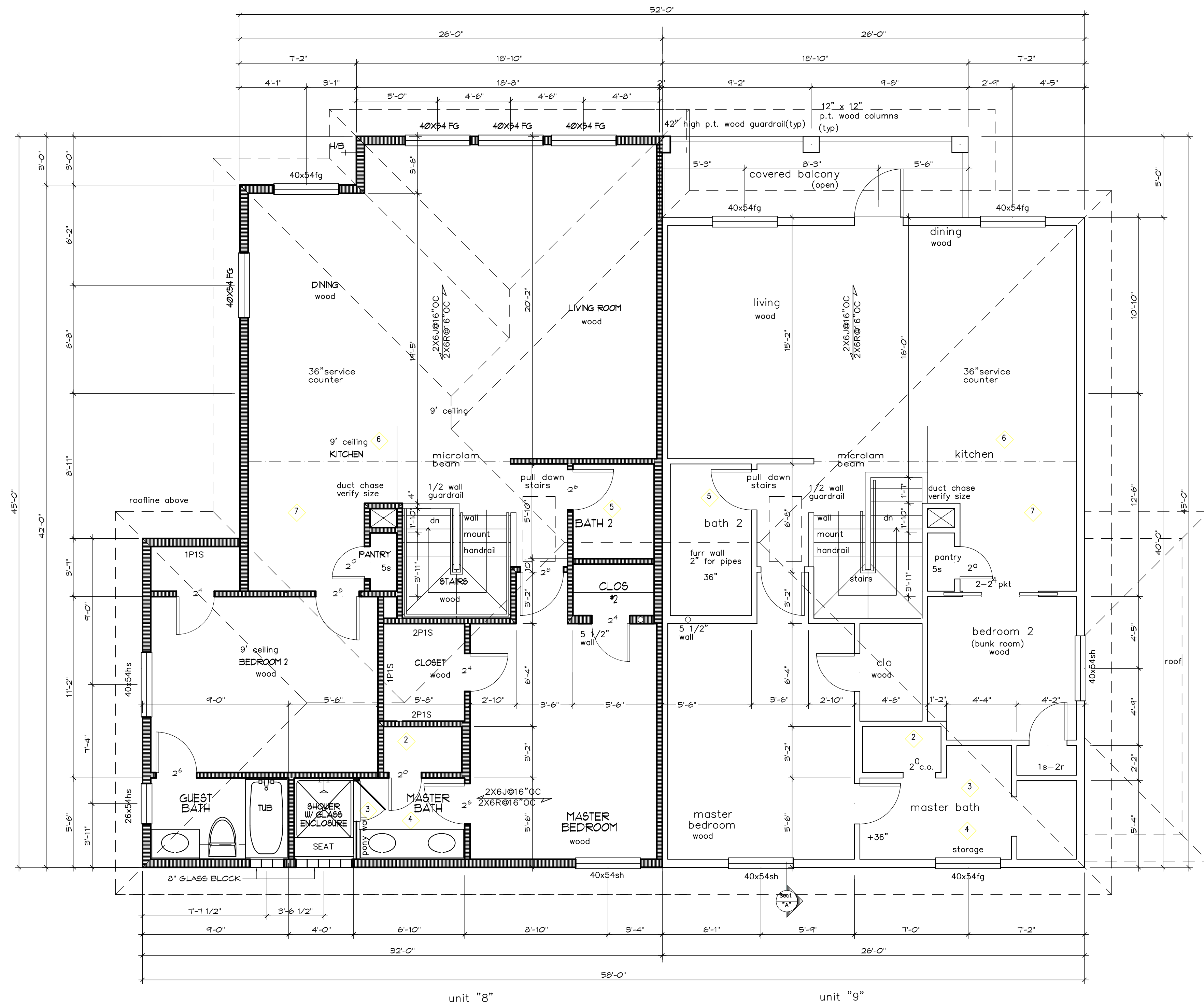
BLDG. "C" 2ND FLOOR PLAN/UNIT "8" OPTION SCALE: 1/4" = 1'-0"
